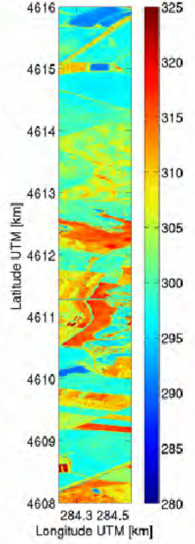
TASI Thermal camera Land Surface Temperature [K]
